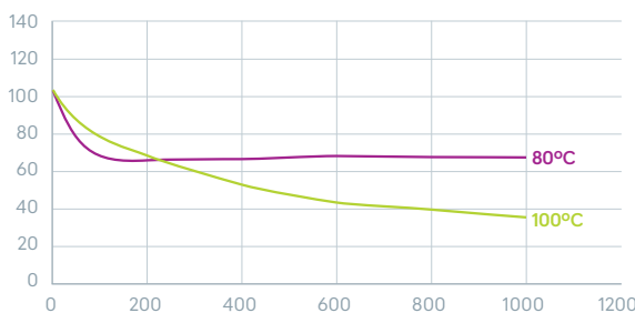
% of Initial Strength = f (Exposure Time (hours))
